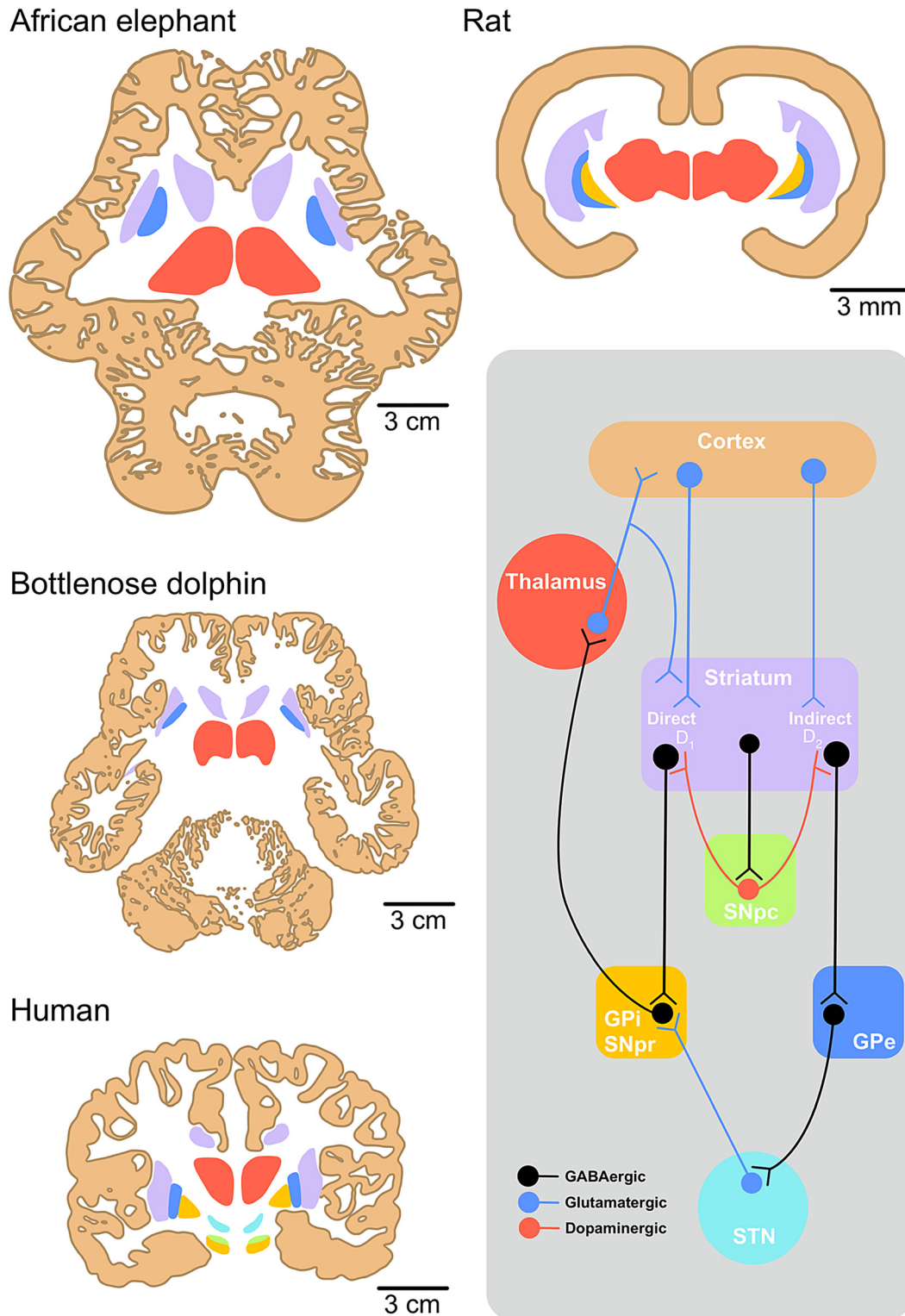
Figure 4: Schematic of brain structures involved in behavioral stereotypes.
