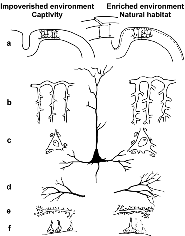
Figure 2: Different levels of the cerebral cortex affected by impoverished (captive) and enriched (natural) environments. In impoverished/captive environments, there are several cortical changes: (a) Decreases in cortical thickness, (b) smaller capillary diameter, (c) decreases in neuronal soma size and fewer glial cells per neuron, (d) less complex dendritic branching, (e) fewer dendritic spines, and (f) less efficient synapses. Image courtesy of Dr. Arnold B. Scheibel.
